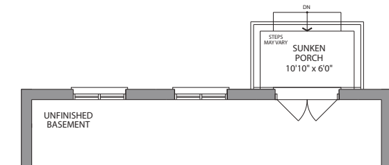
BASEMENT STORM POND UPGRADE ELEVATION A & B
