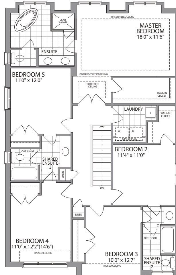
OPT. SECOND FLOOR W/5 BEDROOMS ELEVATION A
