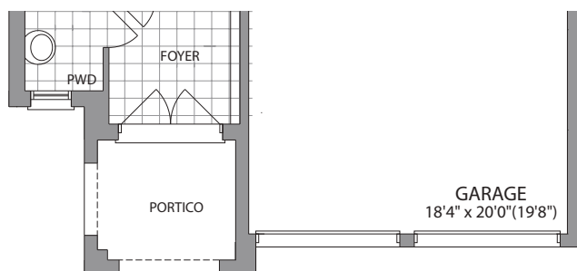
GROUND FLOOR ELEVATION B
